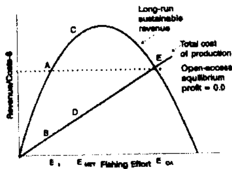
Figure 5. Open-access Equilibrium
